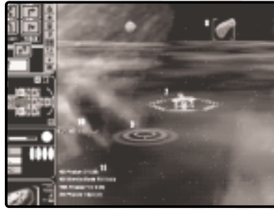
TACTICAL SCREEN
