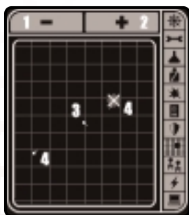
TACTICAL MAP
